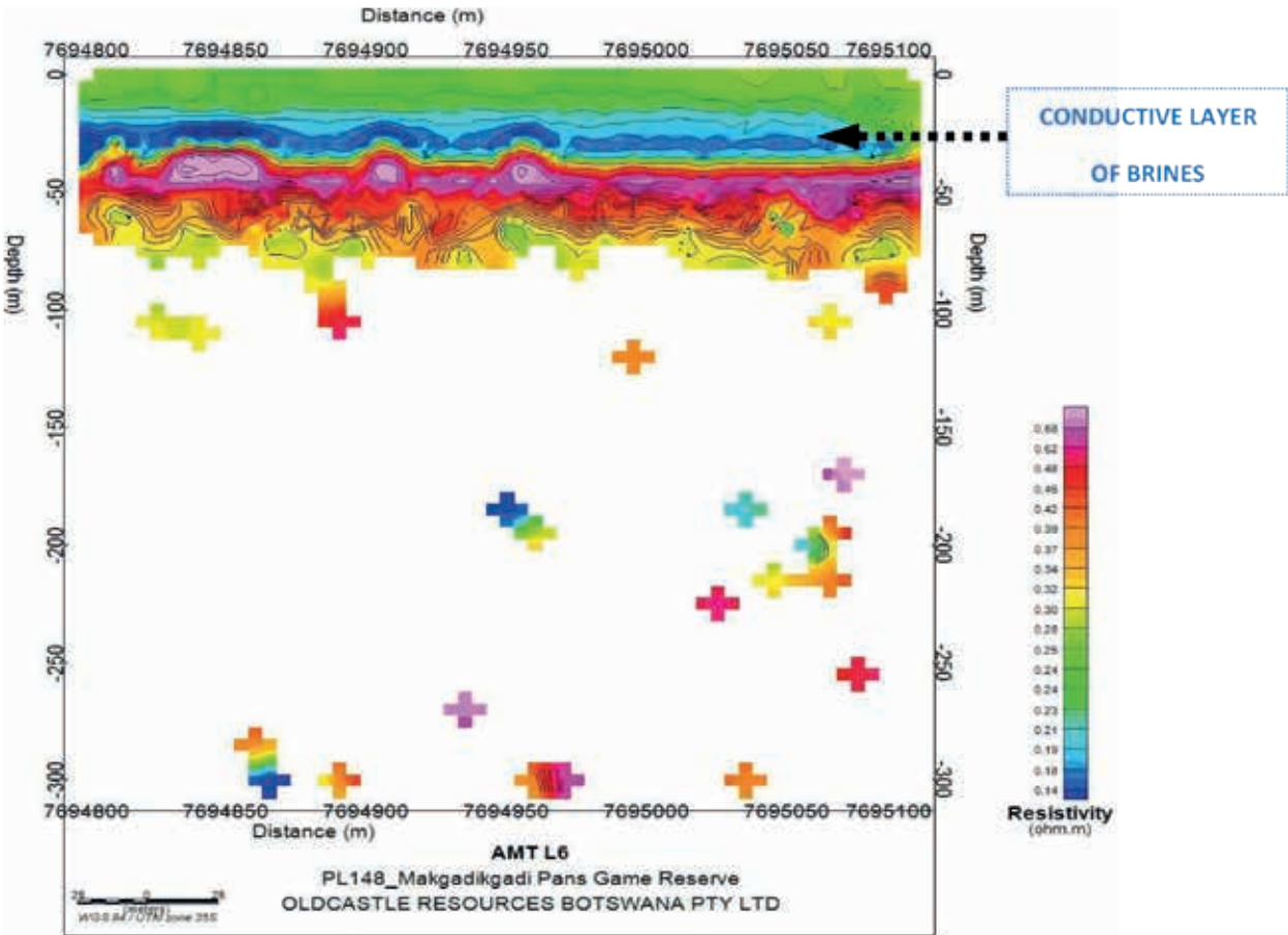
Figure 3-2 2D section of AMT L6 profile on PL148.
