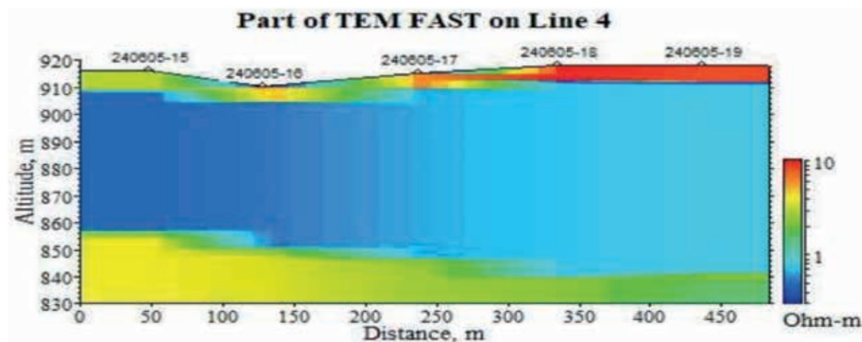
Figure 3-7 A section of TEM FAST line that correspond to area where AMT L8 survey was carried out
