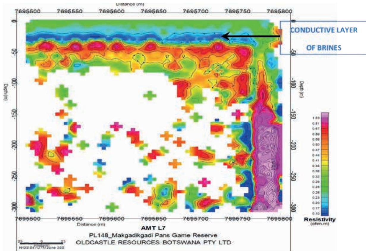
Figure 3-4 2D section of AMT L7 profile line on PL148
