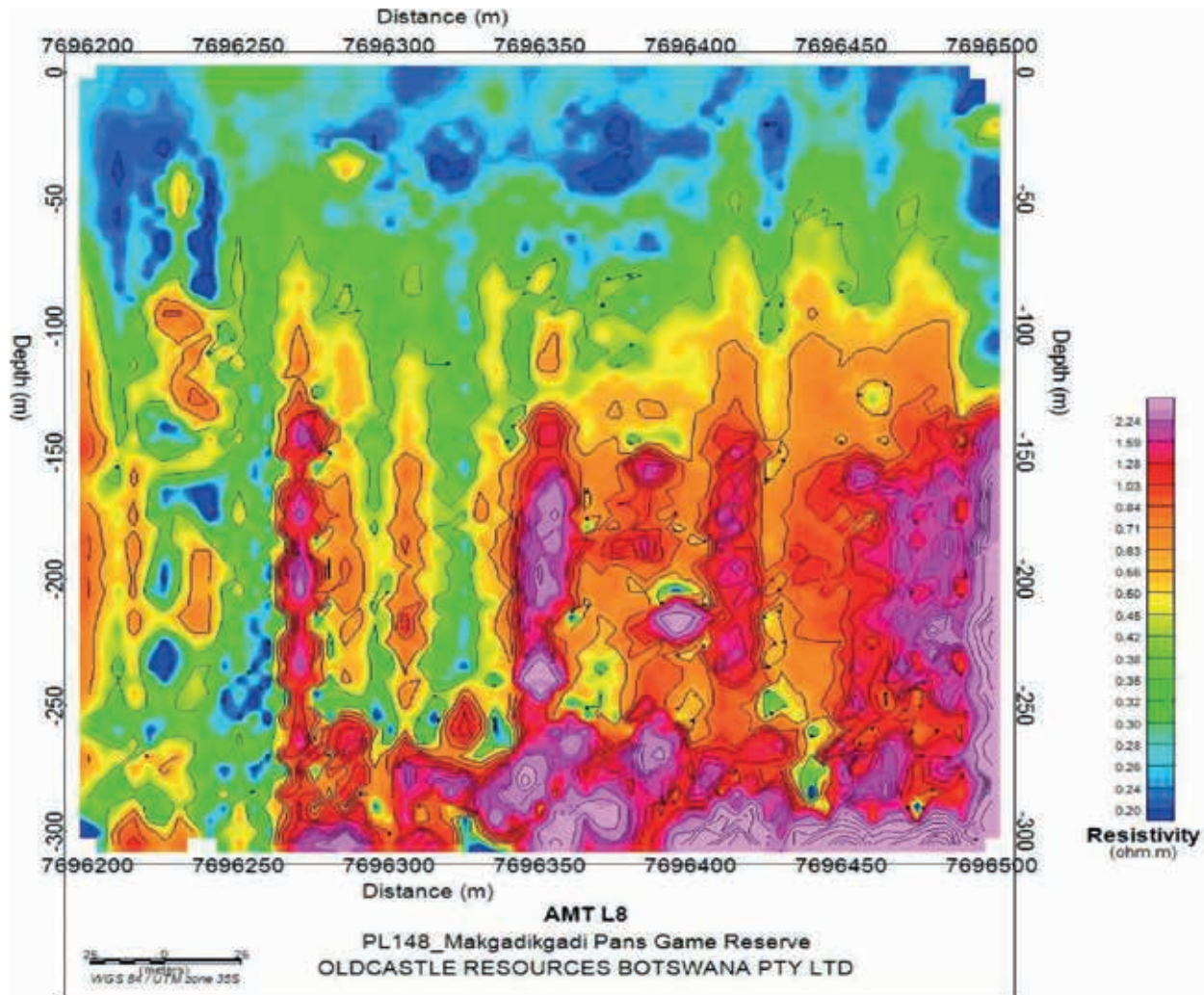
Figure 3-6 2D section of AMT L8 profile line on PL148.
