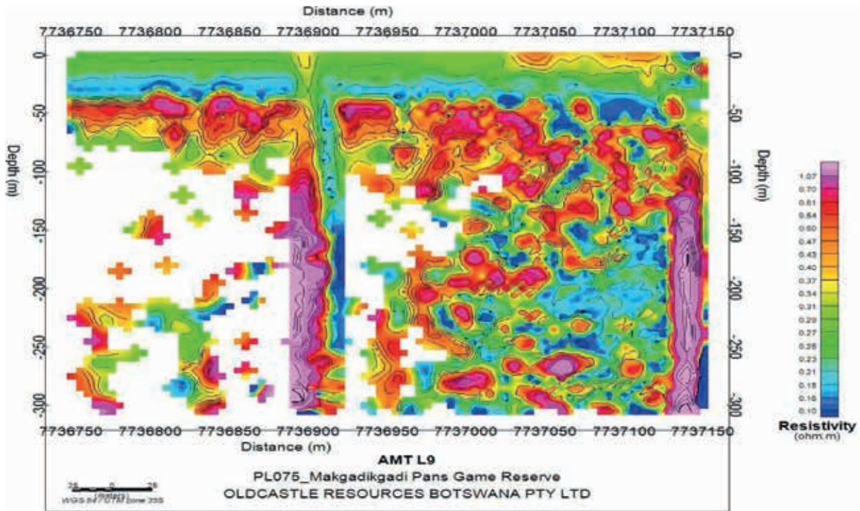
Figure 3-9 2D section of AMT L9 profile line on PL075/2023
