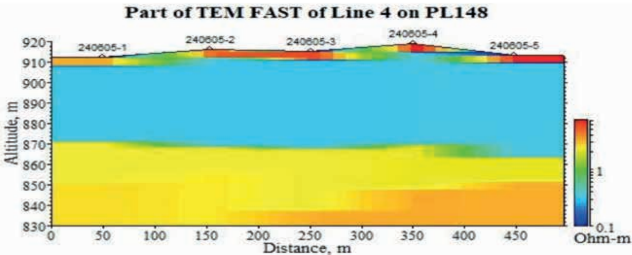
Figure 3-3 A section of TEM FAST line that corresponds to area where AMT L6 survey was carried out.
