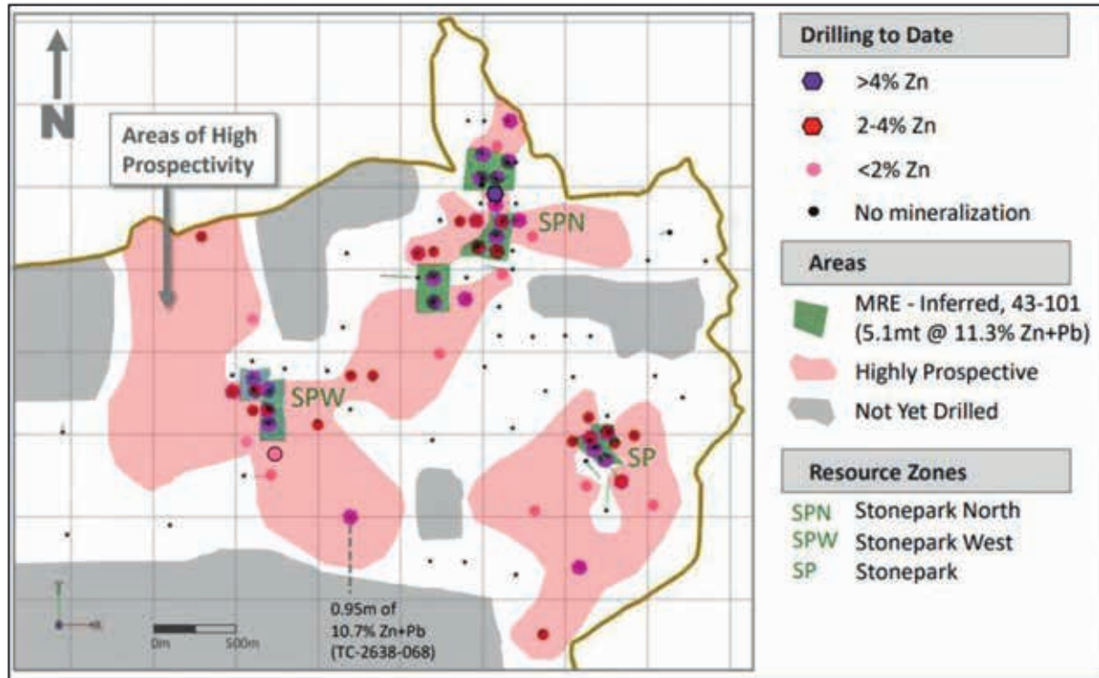
Figure 3 Stonepark deposit (plan view) with extension opportunities (source Group Eleven Resources Corp.)
